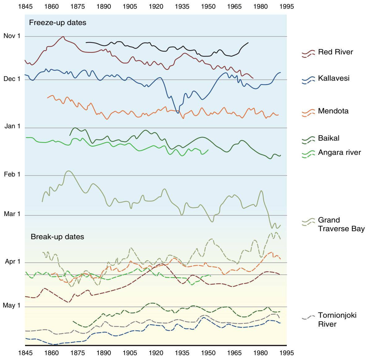
Figure 8.1: Time series of freeze-up and break-up dates from selected Northern Hemisphere lakes and rivers (1846–1995). Data were smoothed with a 10-year moving average.
