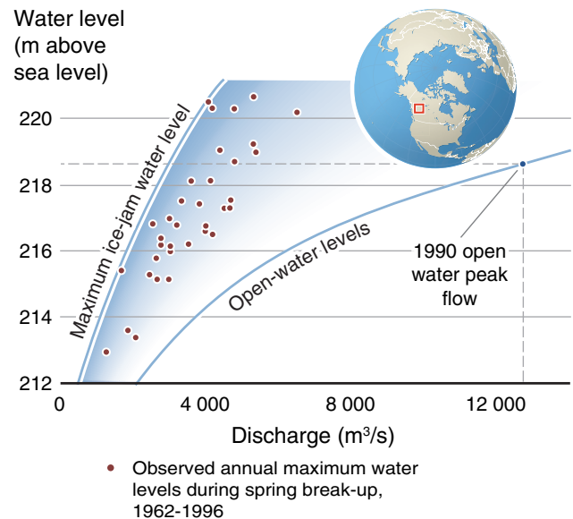
Figure 8.3: Example of enhanced water levels produced from river ice, Liard River (Canada). The lower curve shows the correspondence between river flow and water levels under open-water conditions. The much greater maximum water levels possible under ice-jam conditions are illustrated by the upper curve. The transition in break-up severity from dynamic to thermal break-up effects (see text) is depicted by the gradually shaded area between the two curves. Dots are observed annual maximum water levels during the spring break up. The 1990 dashed line shows the maximum recorded flow for the Liard River – but note that the water level corresponding to this peak flow is lower than for many break-up events with much lower flows. Effects of climate on snowmelt runoff and ice characteristics will lead to regional changes in break-up severity and associated frequency and magnitude of ice-induced flooding.
