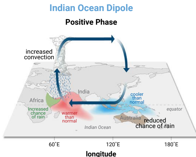
Figure 6: Positive phase of Indian Ocean Dipole.
