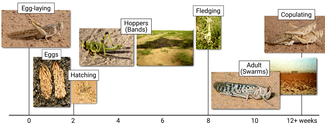
Figure 5: Desert locusts lifecycle. Source: Cressman 2016
