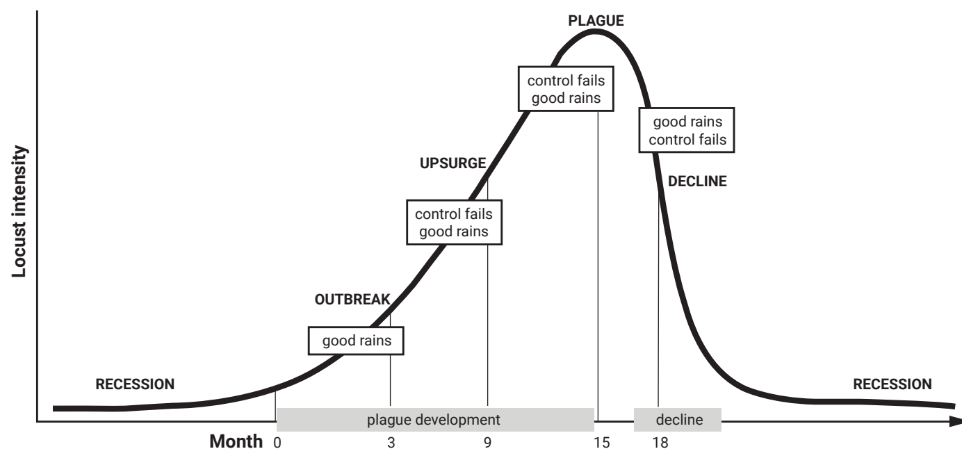
Figure 2: The evolution of desert locust plague. Source: Cressman 2016
