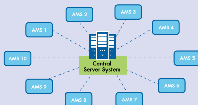
Figure 2: Star-Like Connectivity
