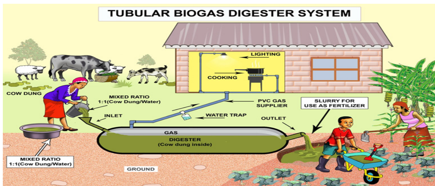
Fig. 01: Plastic Tubular Biogas Digester System
